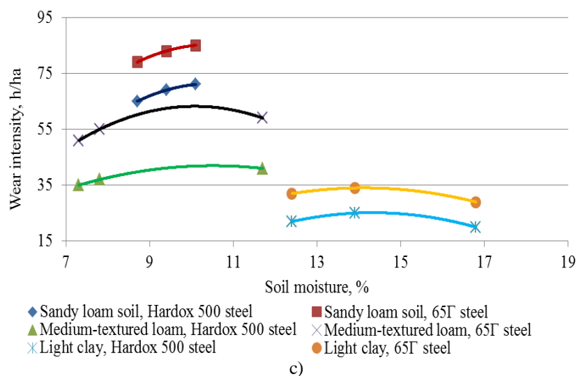
Fig. 4. Impact of soil moisture on wear intensity of the actuating elements of soil processing machines (experimental data): a) – arrowheaded tines. b) – disk actuating elements. c) – bipod
