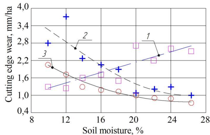
Fig. 3. Impact of soil moisture on wear intensity of the actuating elements of soil processing machines: 1 – sandy soil; 2 – load soil; 3 – clay soil
