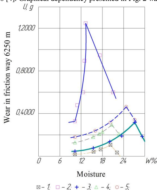
Fig. 2. Dependence of wearability of soils on moisture: 1 – Dark gray light podsollic mid clay loam on forest clay loam. 2 – Common black earth on clay sand. 3 – Light-clay black earth on carbonate forest clay loam. 4 – Dark gray on forest clay loam. 5 – Clay-loam black earth
