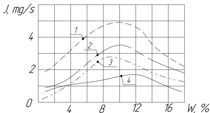
Fig. 1. Dependence of wear intensity on soil moisture: 1 – Sand; 2 – Sandy loam; 3 – Light clay loam; 4 – Clay
