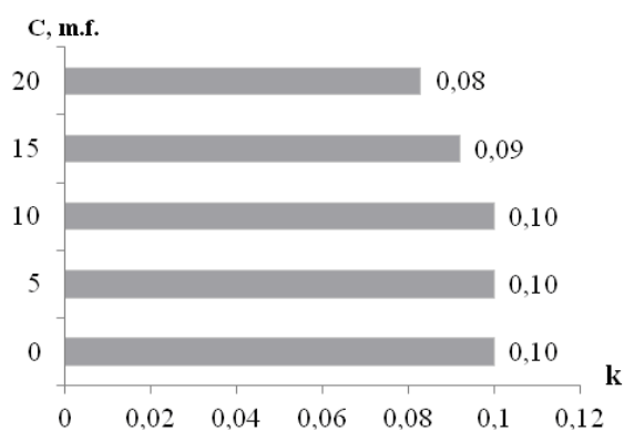
Fig. 6 – Friction coefficient for the developed lubricant with different concentrations of P400 paraffin
