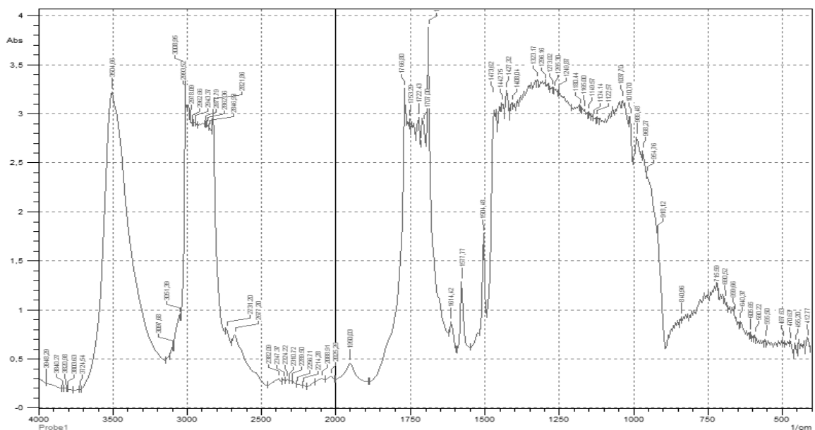
Fig. 4 – IR spectrum of PET-acylglycerol based on beef fat
