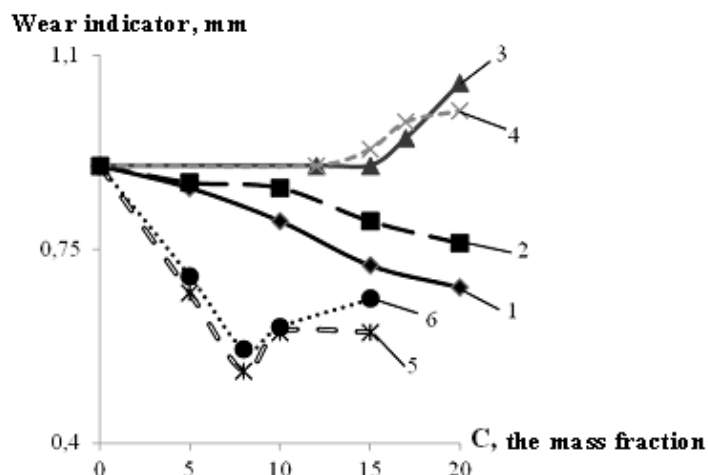
Fig. 5 – Change in wear indicator depending on the concentration of a thickener for a lubricant based on PET-acylglycerol of beef fat:
