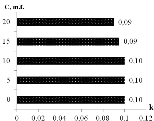
Fig. 7 – Friction coefficient for the developed lubricant with different concentrations of beeswax
