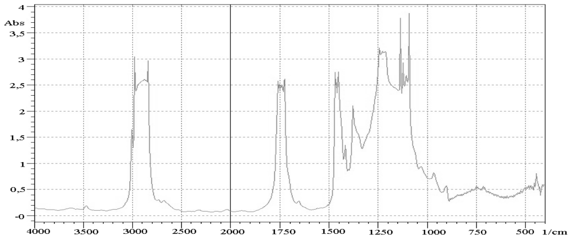
Fig. 3 – IR spectrum of beef fat
