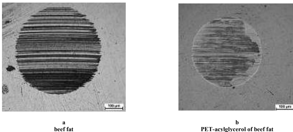
Fig. 12 – Wear traces obtained by means of scanning electron microscopy on experimental balls with a load of 150 N
