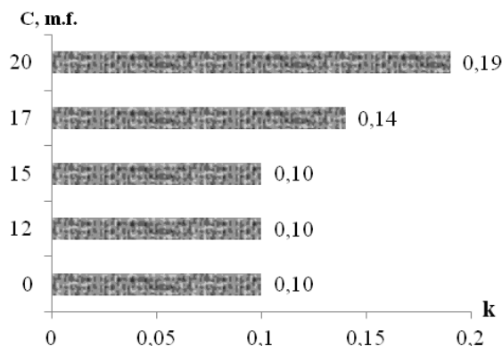
Fig. 8 – Friction coefficient for the developed lubricant with different concentrations of aerosil 200
