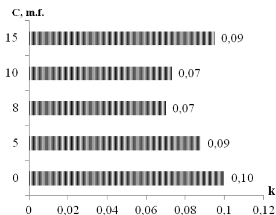
Fig. 11 – Friction coefficient for the developed lubricant with different concentrations of lithium stearate
