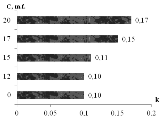
Fig. 9 – Friction coefficient for the developed lubricant with different concentrations of concentrations of bentonite
